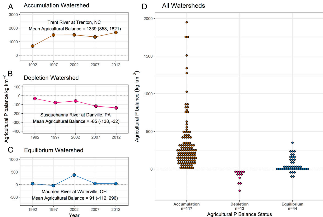
Fig. 2. Examples of watersheds in an (A) accumulation, (B) depletion, and (C) equilibrium status category with the mean of the 5 data points and lower and upper confidence intervals. (D) Mean agricultural P balances for 173 study watersheds by P status category. Each point represents a watershed. N = the number of watersheds within each status category. See Fig. 1B for the geographic locations of the watersheds in each category.
